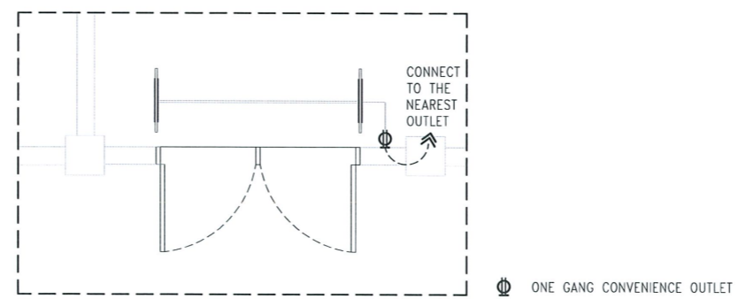
POWER LAYOUT
